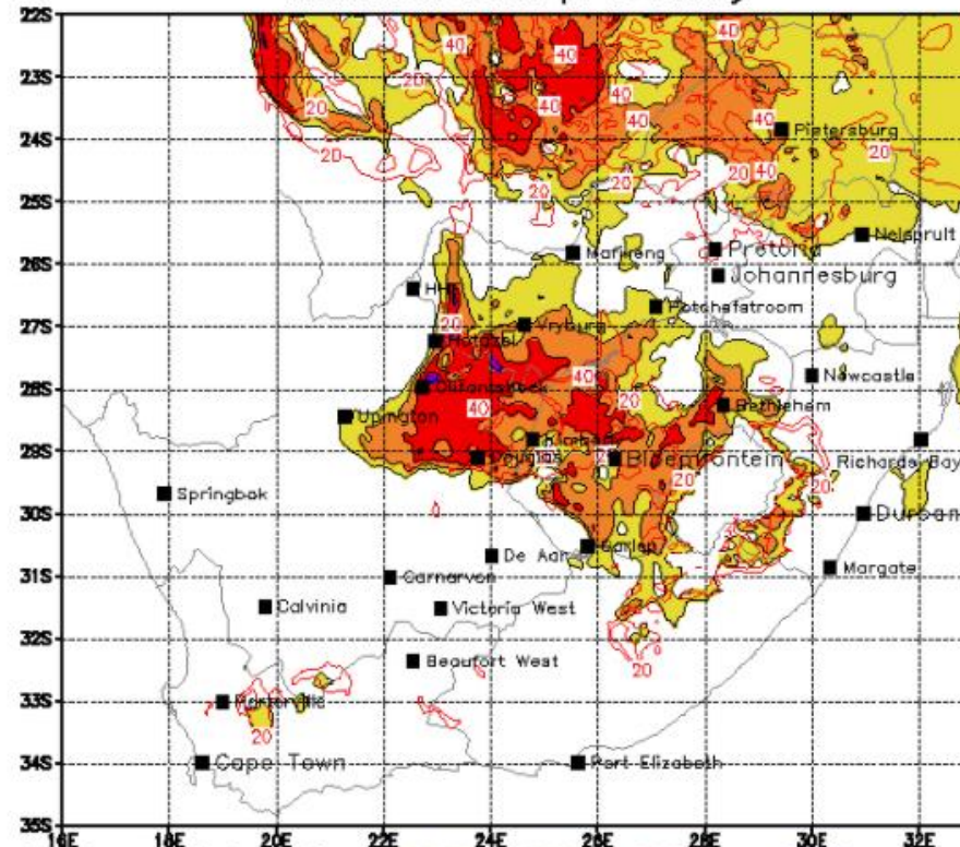
Thunderstorm distribution: 20%; 40%; 60%; >80%; Shaded area=TS prob at 14:00 redlines show 17:00
